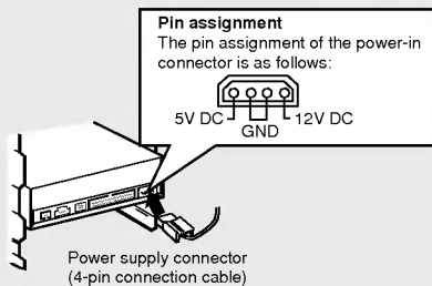
Figure 8. Connecting the Power Supply Cable
