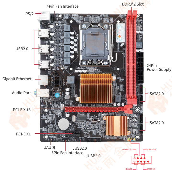
1-1 X58-RX 2.0 Motherboard illustration
