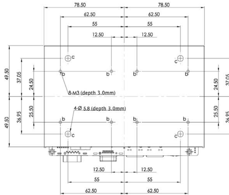
Figure 1-3: Dimensions with Heatsink (mm)
