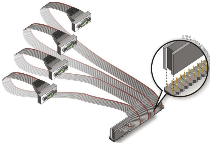
Figure 4-16: Four Serial Port Connector
