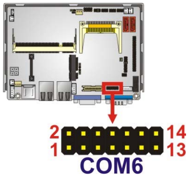
Figure 3-15: RS-232/422/485 Serial Port Connector Location
