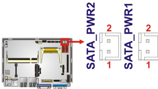
Figure 3-18: SATA Power Connector Locations
