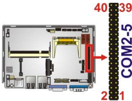
Figure 3-16: RS-232 Serial Port Connector Location
