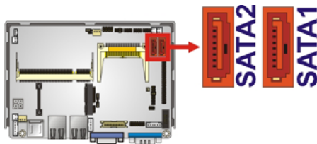
Figure 3-17: SATA Drive Connector Location
