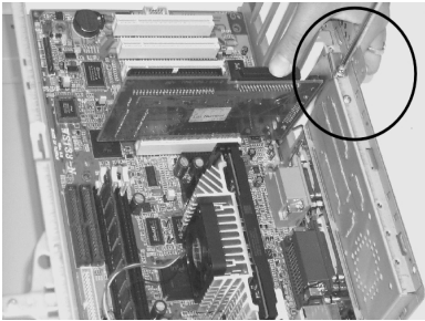
Step 4: Secure the expansion card on the chassis by fastening the screw.
