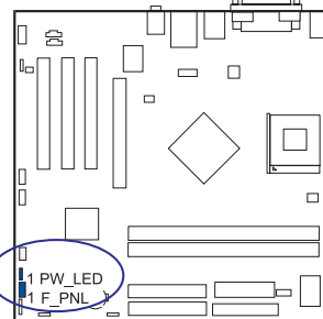
PW_LED (Power LED, 2/3 Pins)
