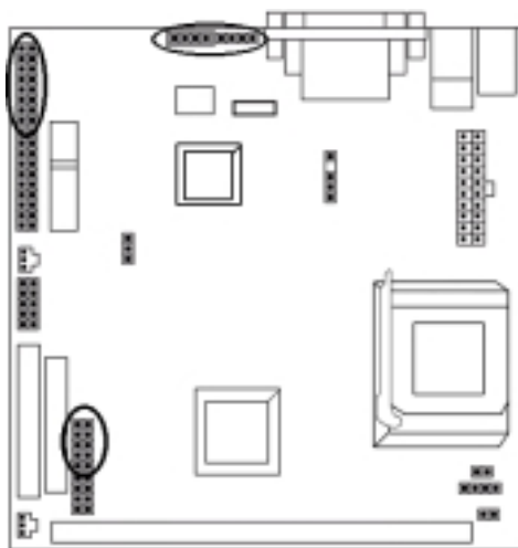
JP1 GAMEPORT
