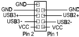
USB (Intel Spec.)
