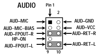
Line-In/Out, MIC Headers
