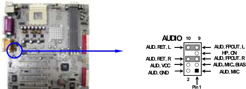
Line-Out, MIC Headers
