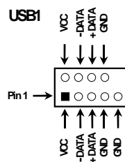
USB Port Connector
