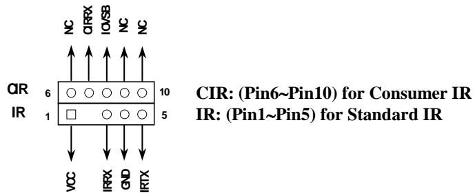
Infrared Module Headers
