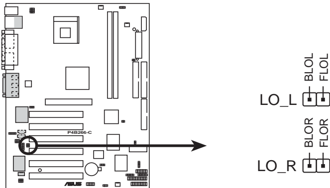
P4B266-C Internal Line Out Connectors
