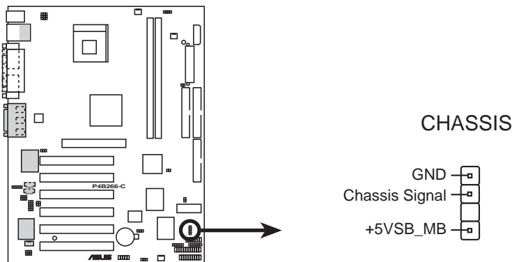
P4B266-C Chassis Alarm Lead
