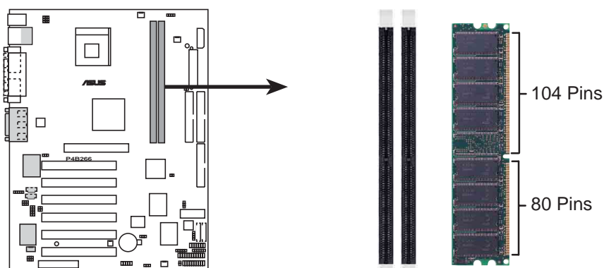
P4B266-C 184-Pin DDR DIMM Sockets
