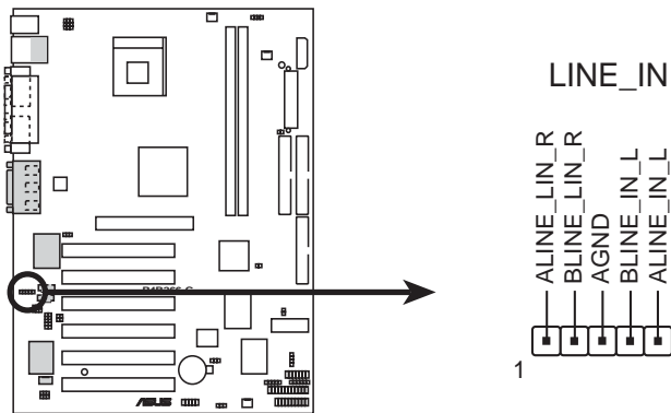
P4B266-C LINE_IN Connector
