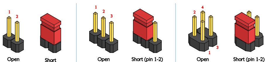
Figure 30: Jumper settings example
