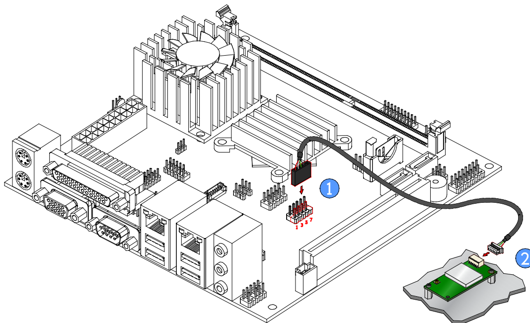
Figure 93: Connecting the USB Wi-Fi cable (VIA EMIO-1533)
