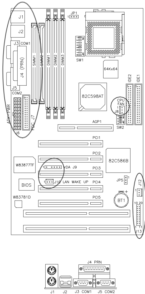
Figure 3: Connector Location on the TI5VG+
