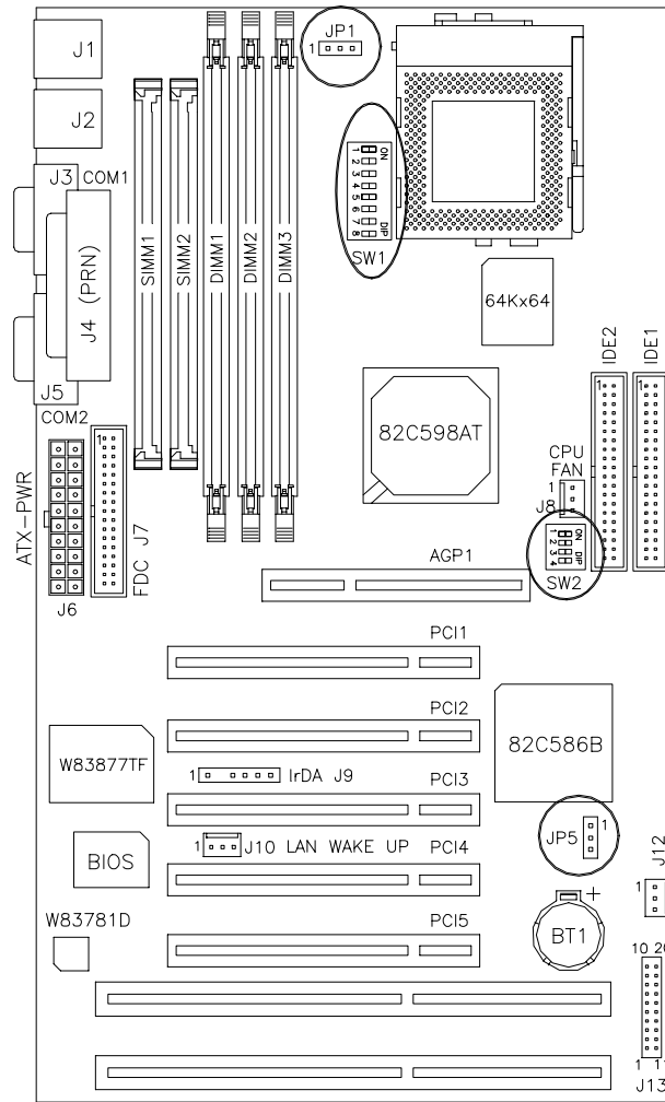
Figure 2: Jumper Locations of the TI5VG+
