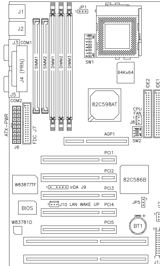
Figure 1: Layout of the TI5VG+ Motherboard
