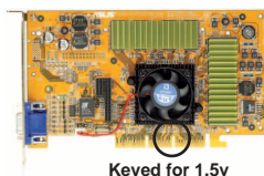
P5S800-VM Accelerated Graphics Port (AGP)
