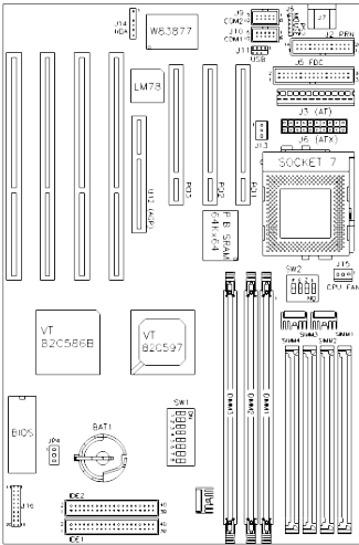
Figure 1: Layout of the SUNRAY VIA AGP Motherboard
