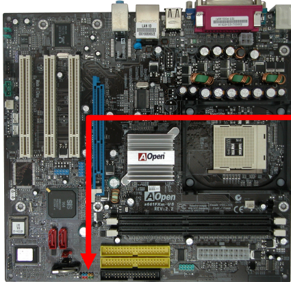
SYSFAN1 Connector
