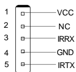
1 IrDA Connector
