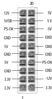
① ATX Power Supply Connector
