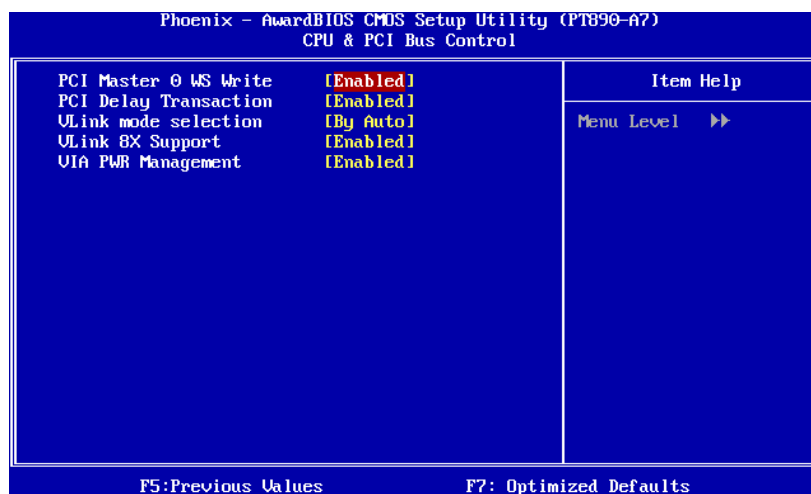
■ Figure 4.2: CPU & PCI Bus Control
