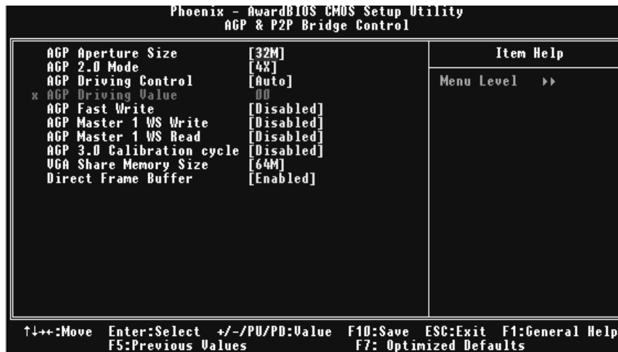
■ Figure 4. 2 AGP & P2P Bridge Control
