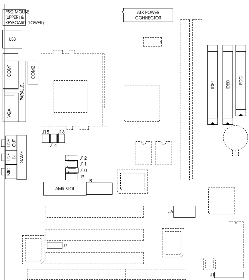
Fig 3 Connector Location
