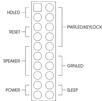
Fig. 4a Multiple Function Jumper
