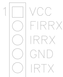
Fig. 8 IrDA Connector
