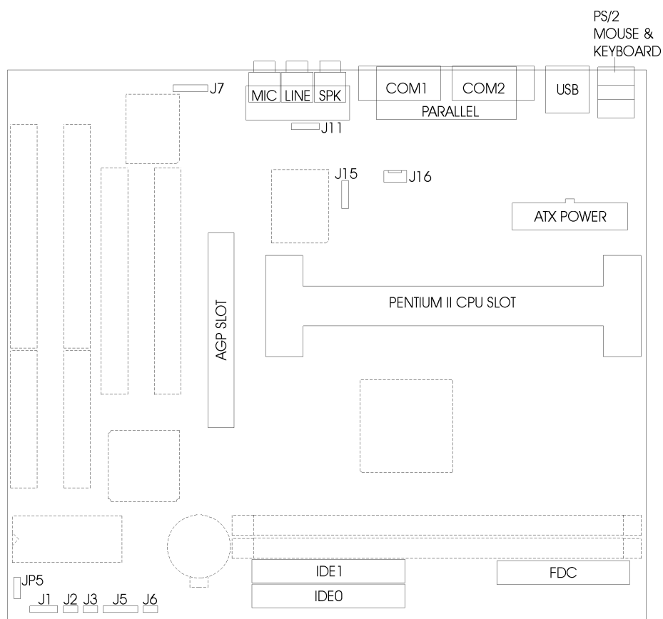
Fig 4 Connector Location
