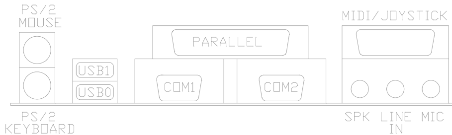
Fig. 14 I/O Connector
