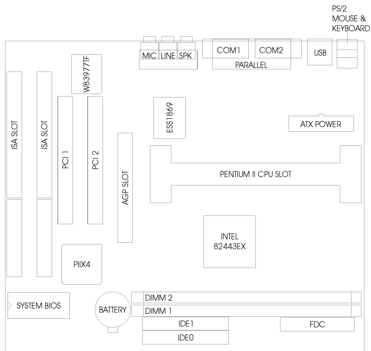
Fig. 1 Key Components of the Mainboard
