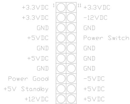
Fig. 13 ATX Power Supply Connector
