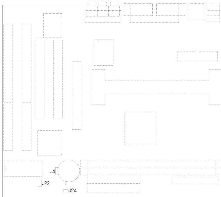
Fig. 2 Jumper Location of the mainboard
