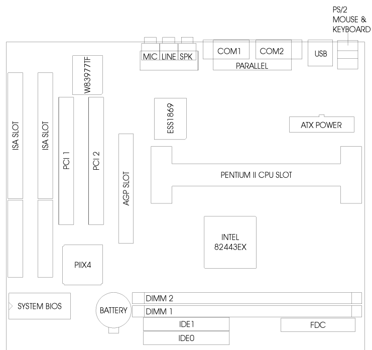
Fig. 1 Key Components of the Mainboard
