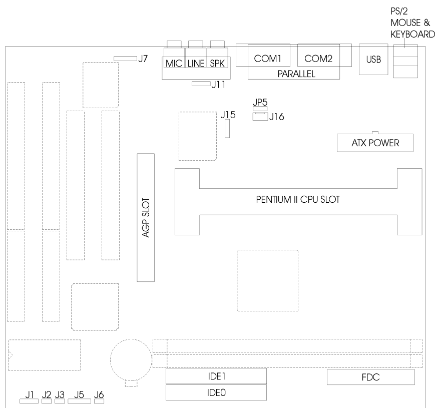
Fig 4 Connector Location
