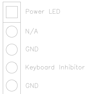
Fig. 6 Keylock Connector
