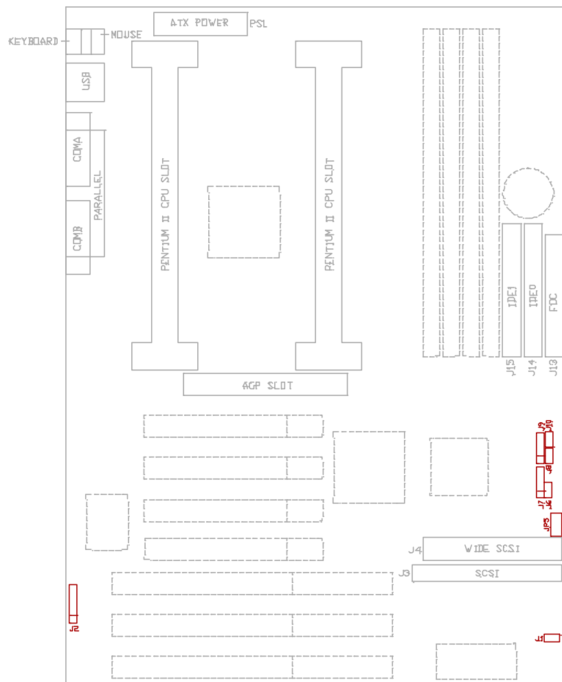
Fig 3 Connector Location
