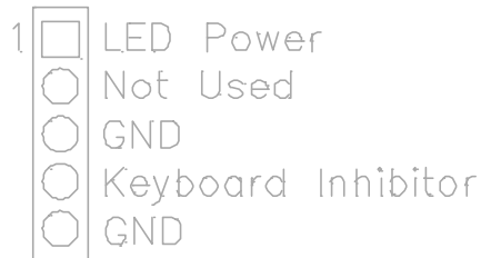
Fig. 8 Power LED
