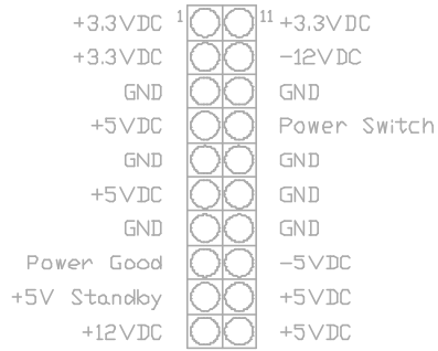
Fig. 4 ATX Power Supply Connector
