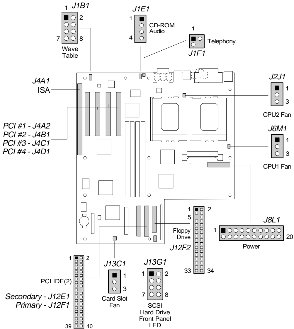
Figure 5. Motherboard Connectors
