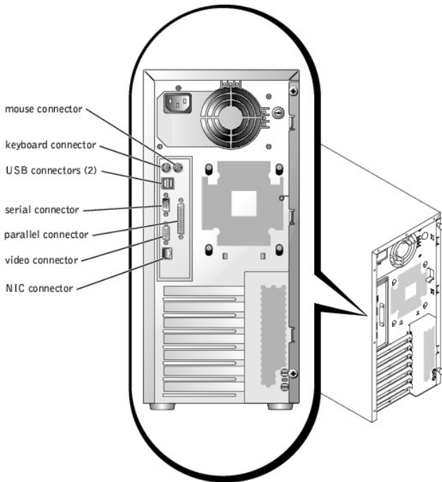
Figure B-1. I/O Ports and Connectors
