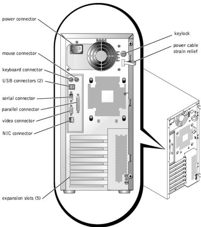
Figure 1-3. Back-Panel Features
