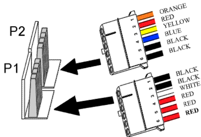
Standard AT Power Supply Connectors
