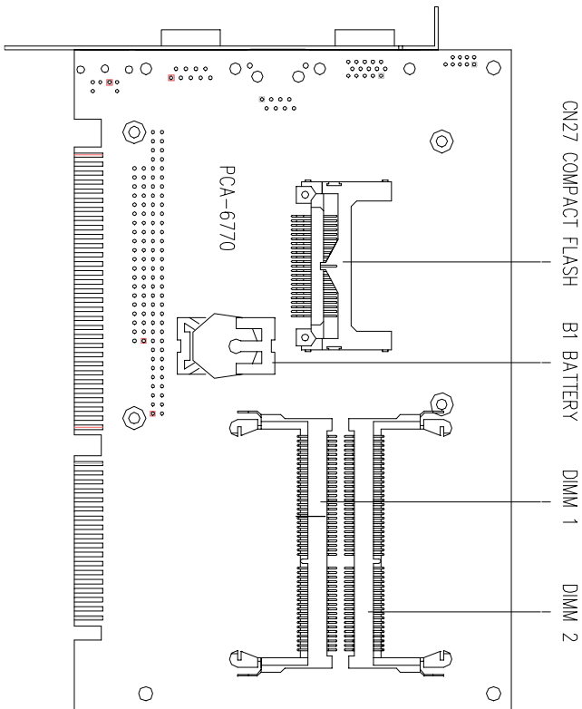
Figure 2-2: Locating connectors (solder side)
