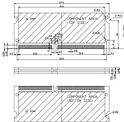
Figure 2-5: Standard SODIMM Dimensions
