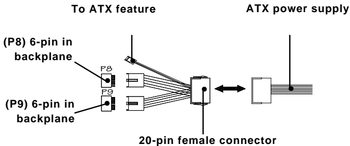
Figure 2-4: ATX Adaptor cable
