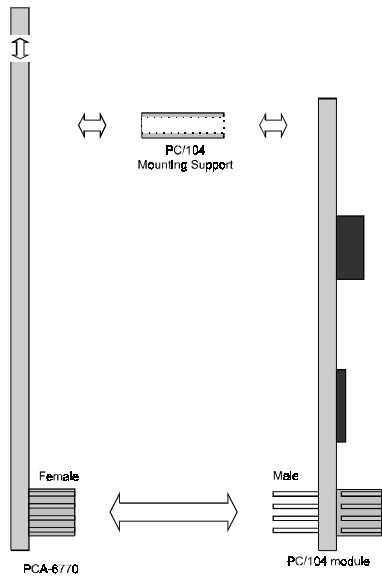
Figure B-1: PC/104 module mounting diagram
