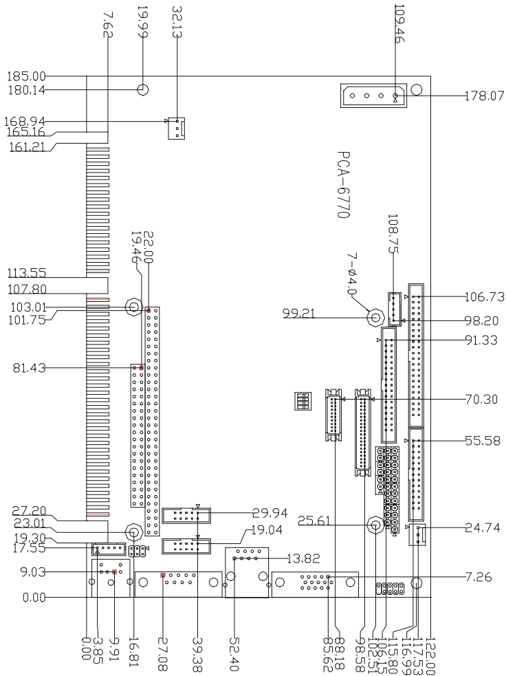
Figure 1-1: PCA-6770 (dimensions)
