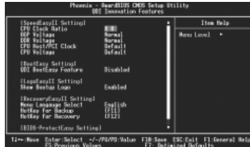
Figure-3 QDI Innovation features Menu
