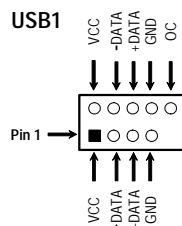
USB2.0 Port Headers
