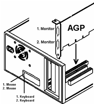
Dual Port AGP VGA Card
