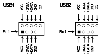
USB Port Headers
