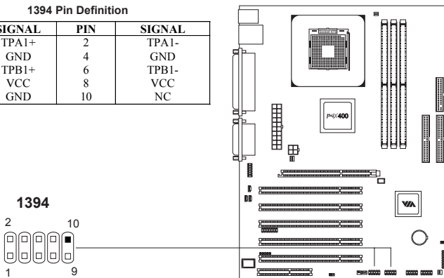
1394 Pin Definition
