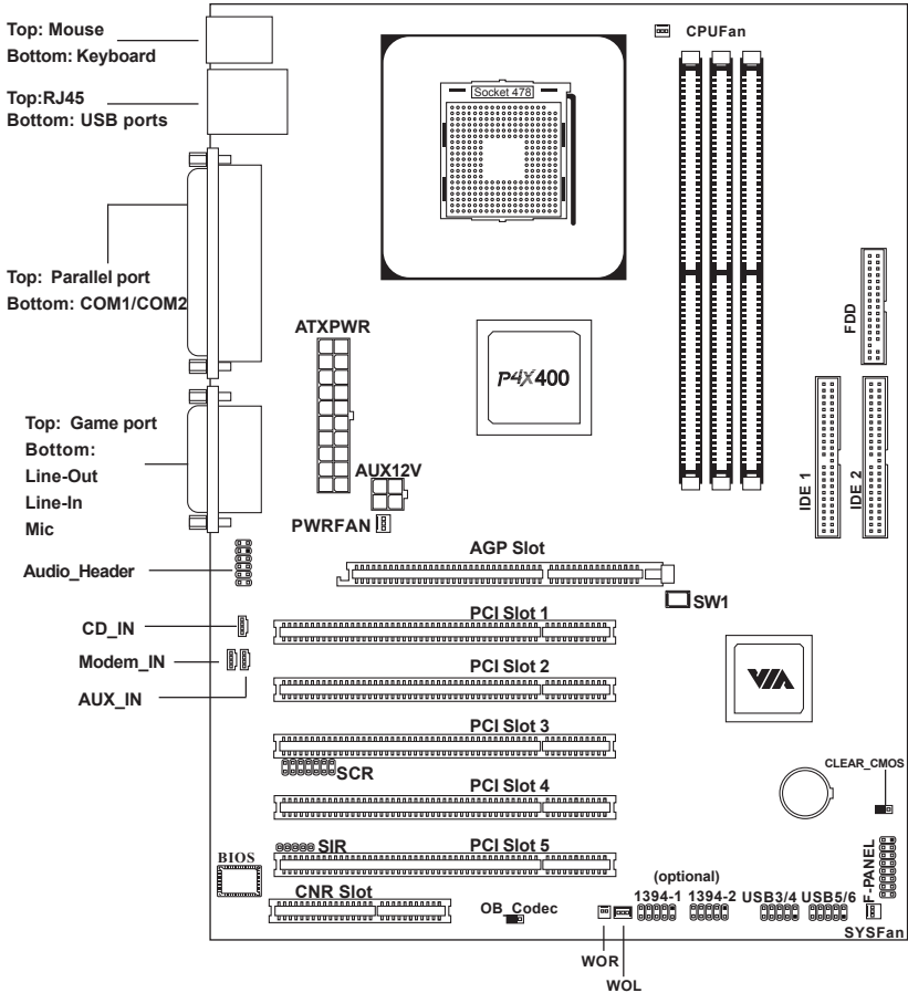
VIA P4PB 400 Mainboard
