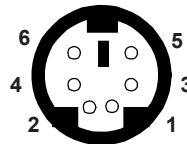
PS/2 Keyboard (6-pin Female)
