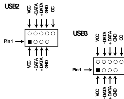
USB Port Headers
