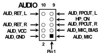
Line-In/Out, MIC Headers
