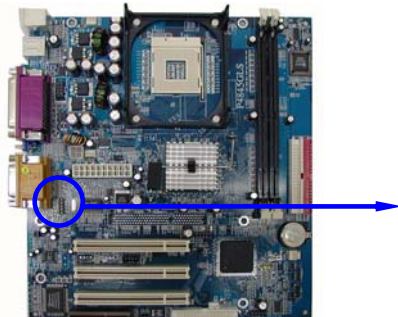
Line-In/Out, MIC Headers
