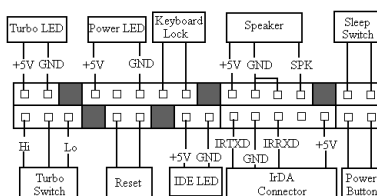
JFRNT Panel Connector
