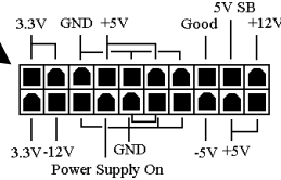
J1 ATX Power Connector
