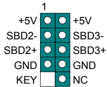
USB2 Connector
