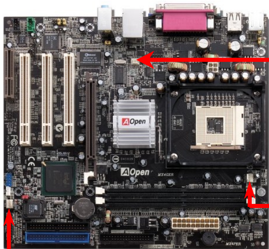
SYSFAN3 Connector
