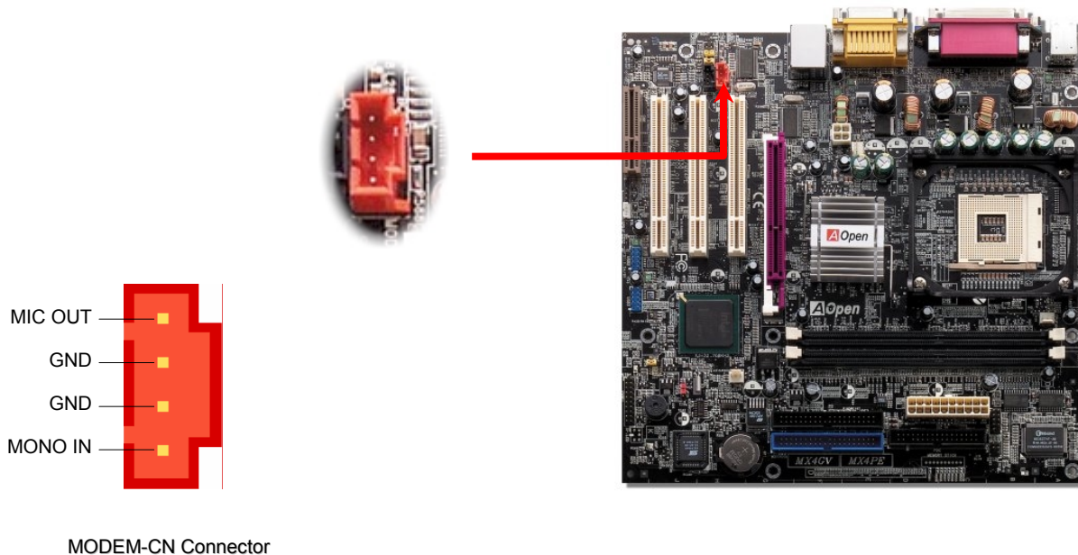
MODEM-CN Connector
