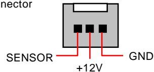
FAN3 Connector
