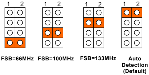
JP23 FSB Select Jumper
