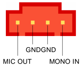
MODEM-CN Connector
