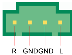
AUX-IN Connector
