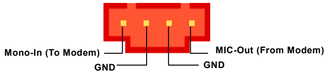
MODEM-CN
