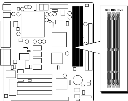
Figure 4-1 : MB11/MZ11 provides three DIMM sockets
