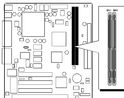
Figure 4-2 : provides two DIMM sockets
