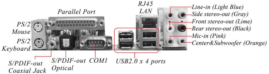
Figure 10 - I/O Ports
