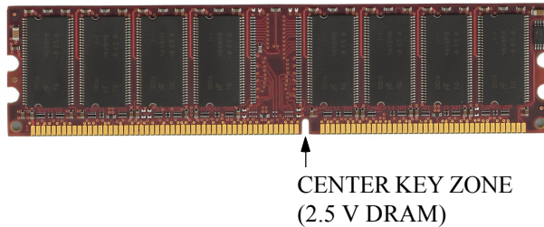
<Figure 7> DIMM notch
