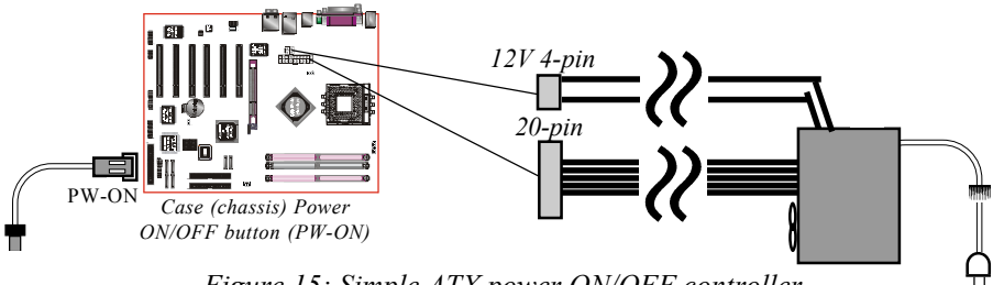
Figure 15: Simple ATX power ON/OFF controller
