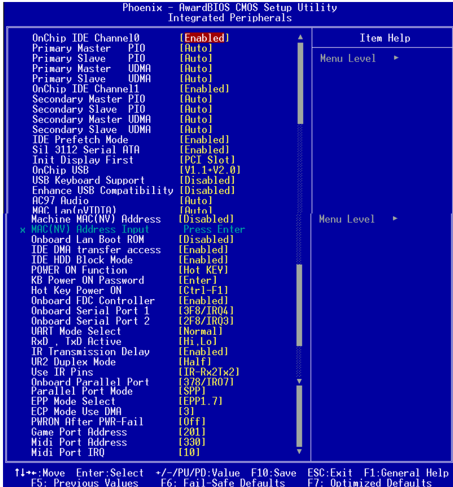
Figure 5: Integrated Peripherals
