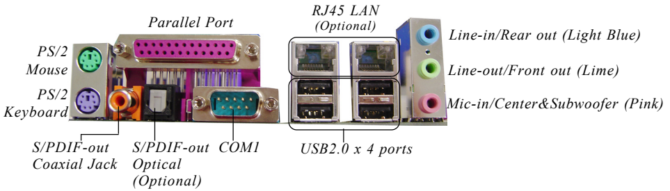
Figure 10 - I/O Ports
