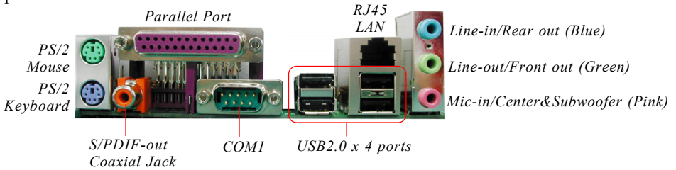
Figure 10 - I/O Ports
