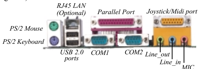
Figure 3: I/O ports
