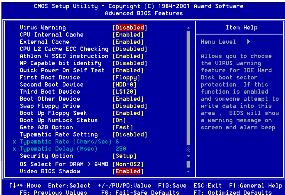
Figure 3: BIOS Features Setup
