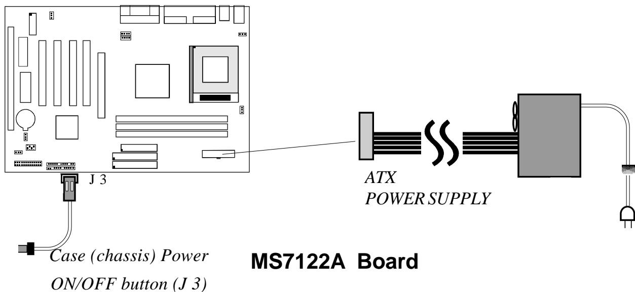
Figure 4: Simple ATX Power ON/OFF Controller
