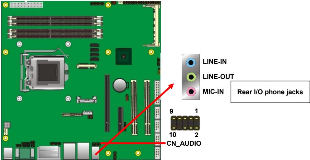
Connector: CN_AUDIO Type: 10-pin (2 x 5) header
