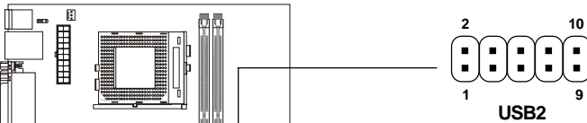
Pin Definition
